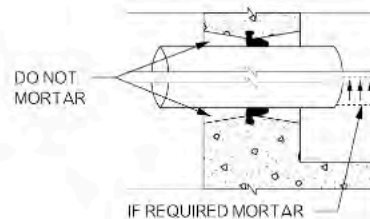
INVERT INSTALL A-LOK CONNECTOR SYSTEM
